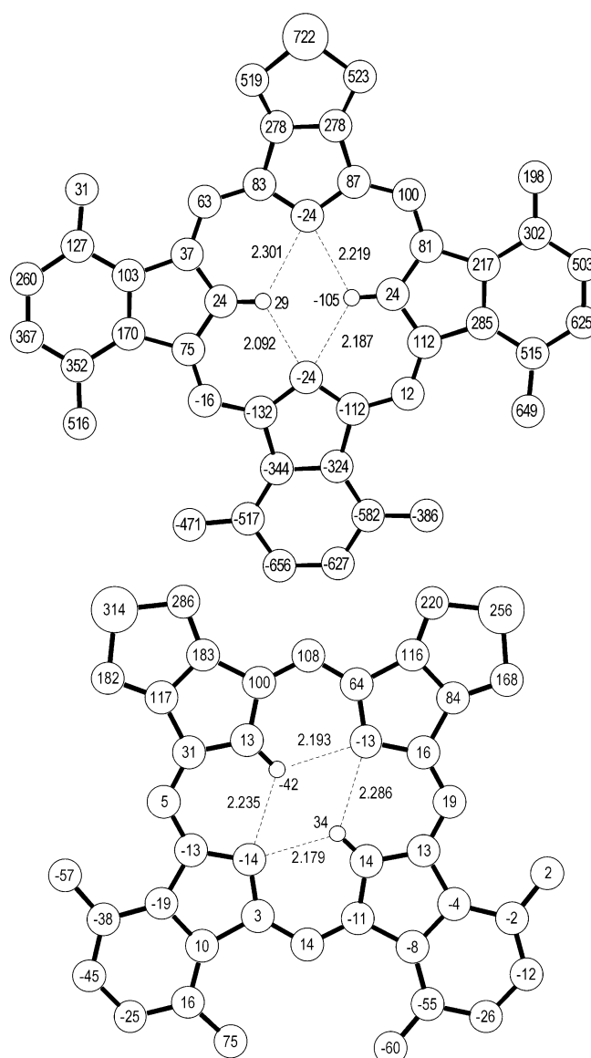
Figure 3. Deviations of atoms [ 10^3 \text{ \AA} ] constituting the macrocyclic skeleton in (SA_3)PzH_2 (top) and (S_2A_2)PzH_2 (bottom) from the mean N_4 plane formed by internal nitrogen atoms and intramolecular hydrogen bonds [ \text{\AA} ].
