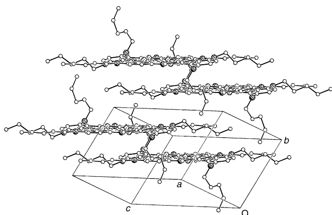
Figure 7. The packing of (A_4)PzH_2 (SCHAKAL view). Disorder affecting some alkyl chains has been omitted for clarity.
