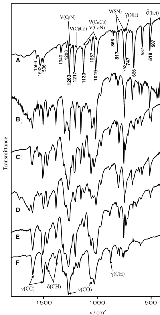
Figure 8. IR spectra of (S_3)PzH_2 (A), (S_3A)PzH_2 (B), (S_2A_2)PzH_2 (C), (SASA)PzH_2 (D), (SA_3)PzH_2 (E), and (A_4)PzH_2 (F). For (S_3)PzH_2 , bold-type wavenumbers indicate vibrations of 1,2,5-thiadiazole rings and, strongly coupled with them, pyrrole ring vibrations. The assignments for vibrations of the amyloxy groups are shown for (A_4)PzH_2 .
