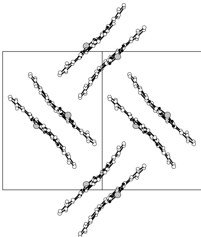
Figure 6. View of the unit cell of (S_3A)PzH_2 along the (101) axes. Alkyl chains are omitted for clarity.
