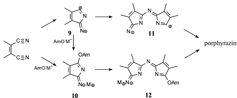
Scheme 3. Possible mechanisms for the formation of porphyrazine macrocycles.
